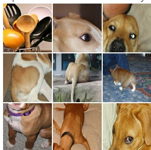
Dataset examples
